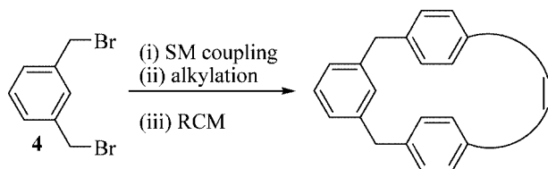
Scheme 1. Synthetic strategy for cyclophane synthesis.
