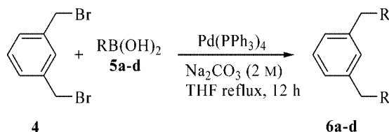
Scheme 2. The reaction was conducted with the boronic acid (1.5 equiv. for each bromine atom in the substrate), Pd(PPh 3 ) 4 (6–10 mol-%).
