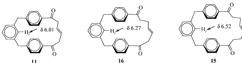
Figure 2. Magnetic anisotropic effects in various cyclophane derivatives.
