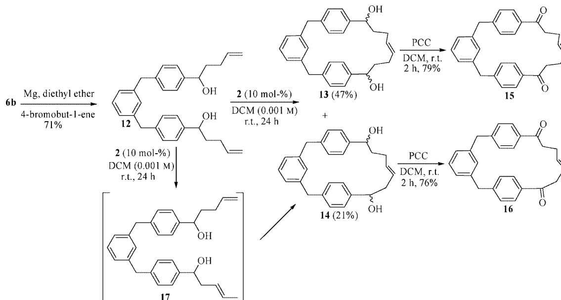
Scheme 5. Synthesis of higher analogues of 11 .
