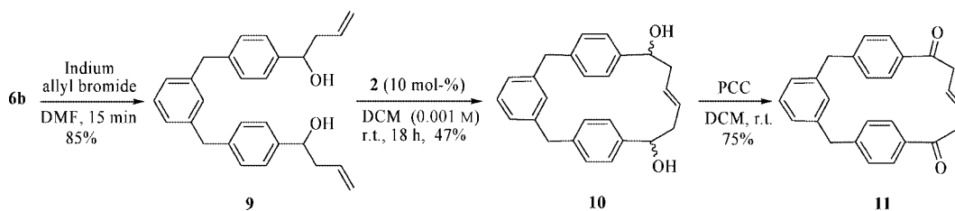
Scheme 4. Synthesis of 11 with RCM as a key step.
