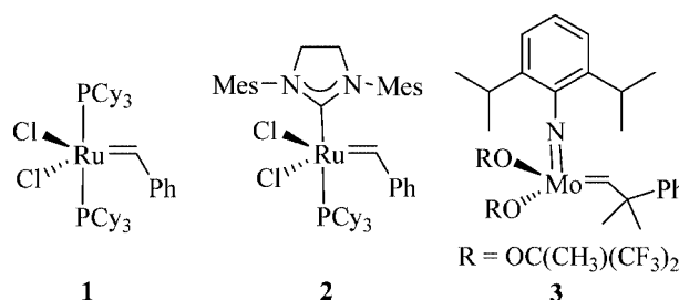
Figure 1. Commonly used olefin metathesis catalysts.
