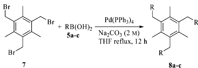
Scheme 3. The reaction was conducted with boronic acid (1.5 equiv. for each bromine atom in the substrate), Pd(PPh 3 ) 4 (10–15 mol-%).
